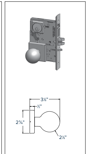
BALL KNOB — KJSR
