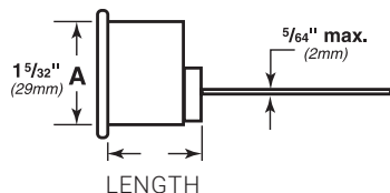
RIM CYLINDER
