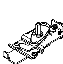
Signal Switch / REX With Dogging
